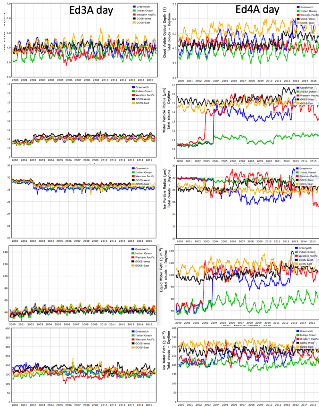
Figure 4-4. Same as Figure 4-3 except for the daytime total cloud visible optical depth, cloud water particle radii, cloud ice particle radii, liquid water path and ice water path.
