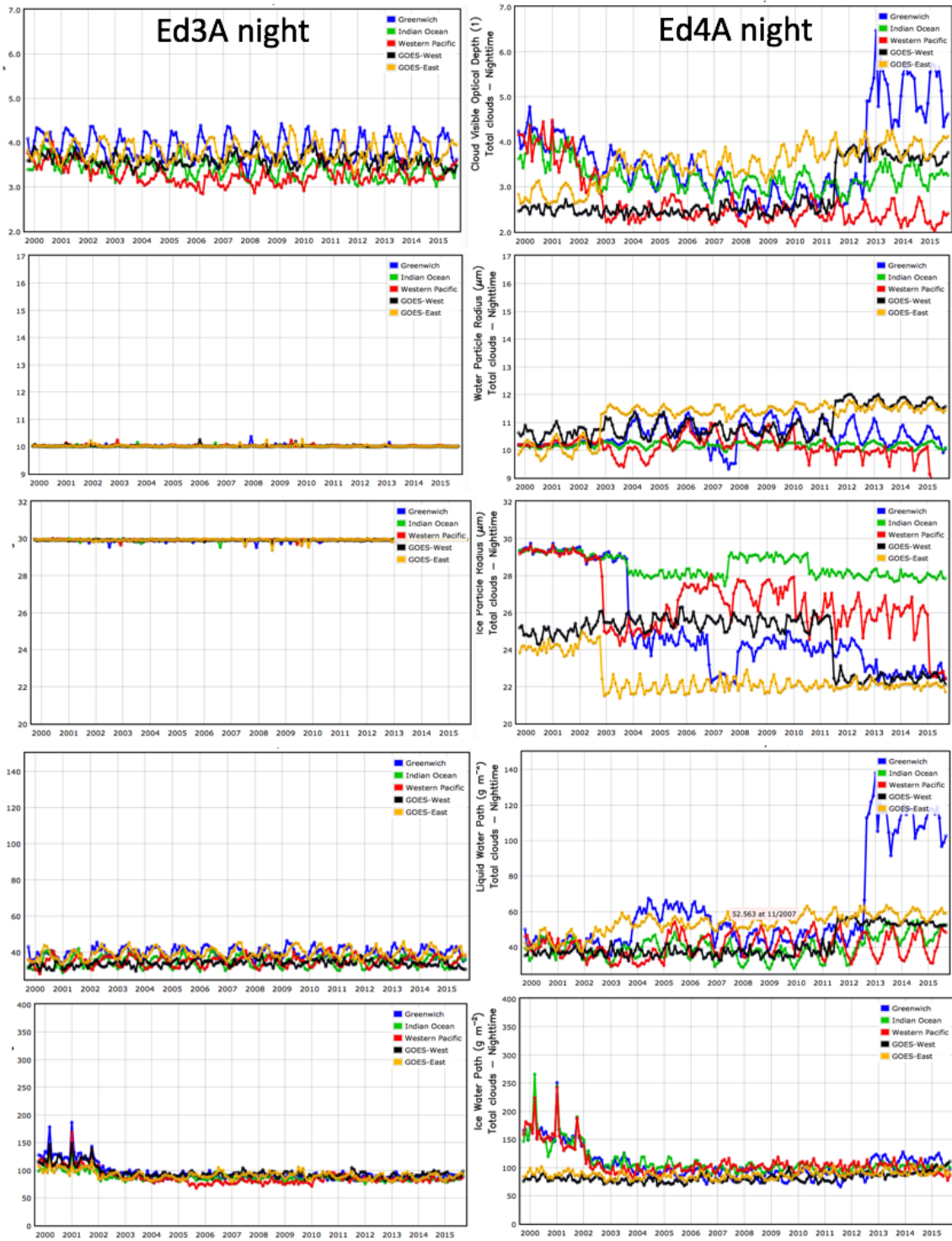
Figure 4-6. Same as Figure 4-3 except for the nighttime total cloud visible optical depth, cloud water particle radii, cloud ice particle radii, liquid water path and ice water path.
