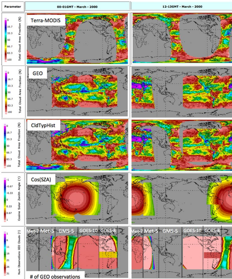
Figure 1-5. The March 2000 monthly 0-1 GMT hourly (left panel plots) and 12-13 GMT (right panel plots) mean cloud amount for Terra-MODIS, GEO-only, CldTypHist or Terra-MODIS and
