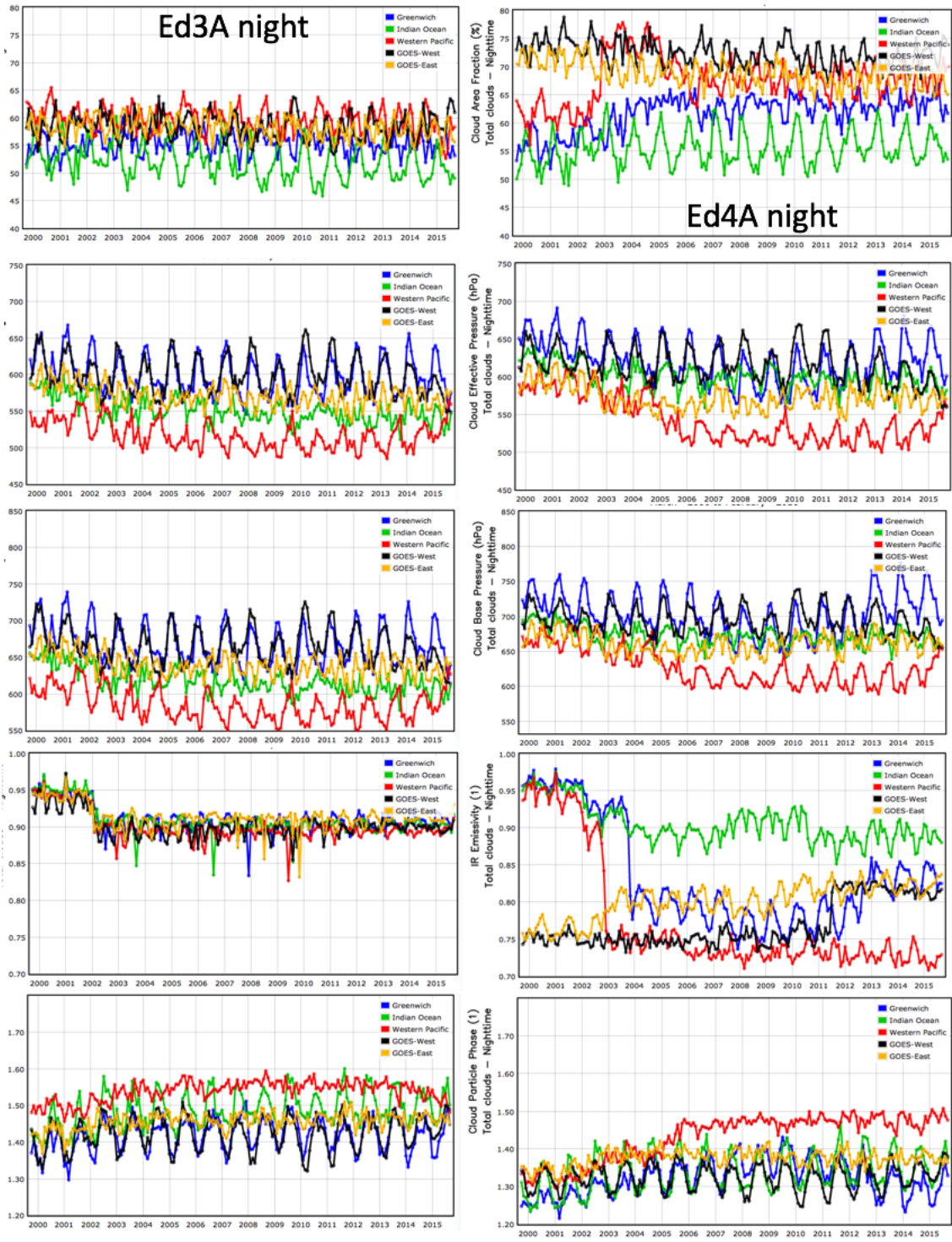
Figure 4-5. Same as Figure 4-3 except for the nighttime total cloud fraction, cloud effective pressure, cloud base pressure, IR emissivity, and cloud phase.
