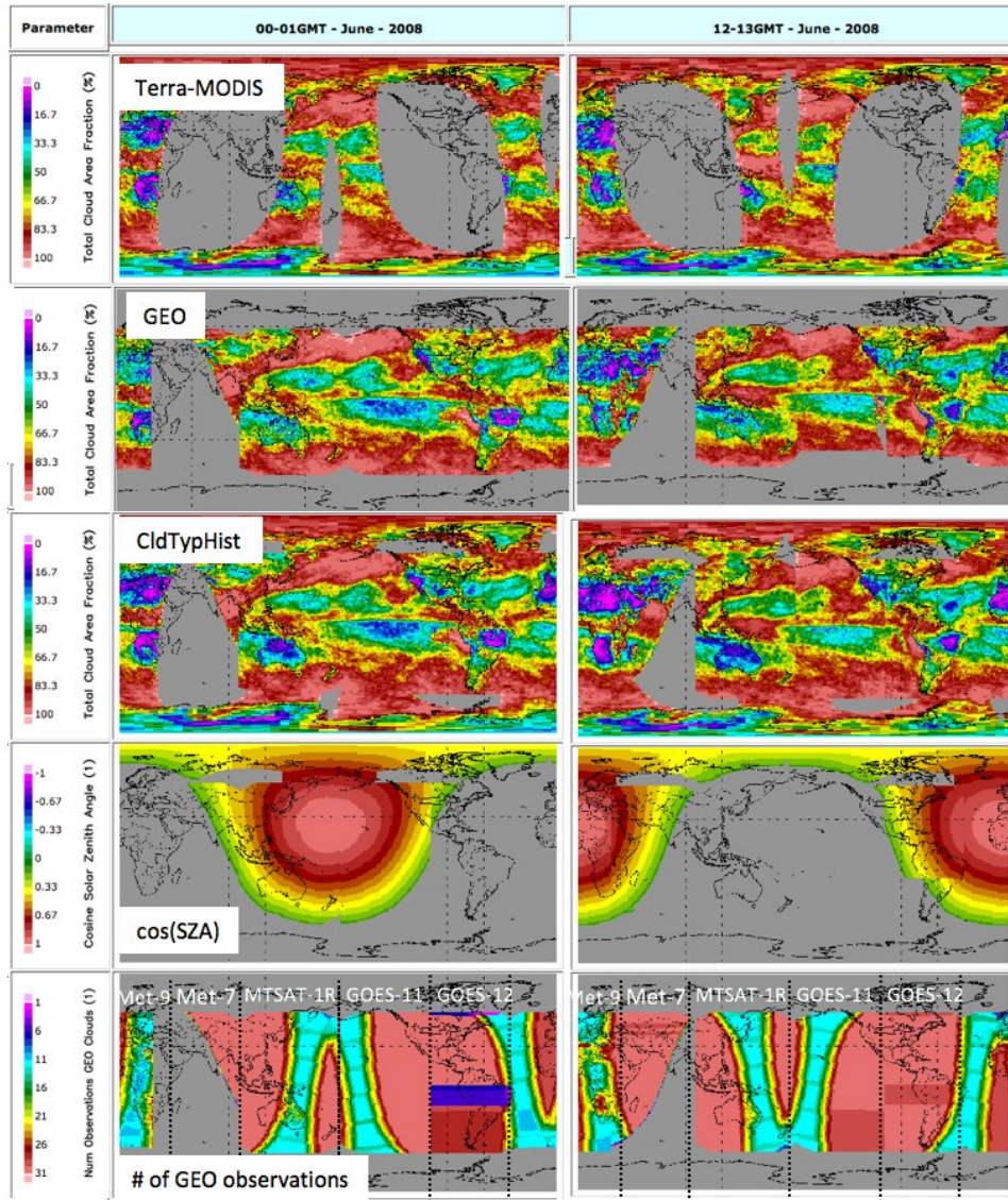
Figure 1-6. Same as Figure 1-5, except for June 2008. Met-7 is a GEO-2ch satellite and does not provide nighttime cloud properties, whereas the remaining satellites are GEO 5-ch and provide nighttime cloud properties for the product.
