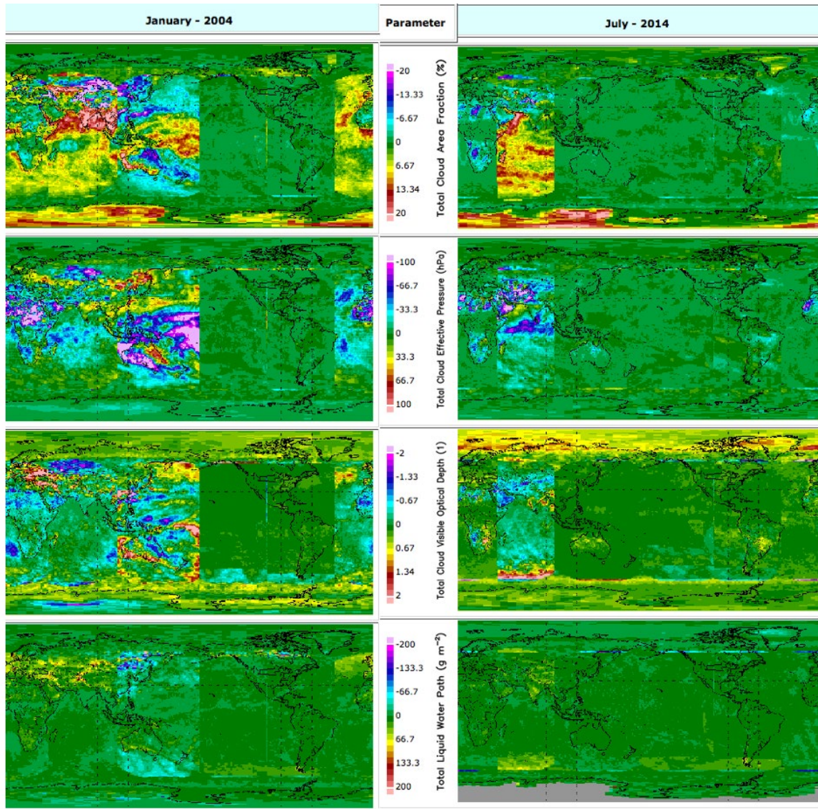
Figure 4-1. The CldTypHist Ed4A minus SYN1deg Ed4A total cloud fraction (%), effective pressure (mb), optical depth, and liquid water path ( \text{g m}^{-2} ). For January 2004 (left panels) and July 2014 (right panels).
