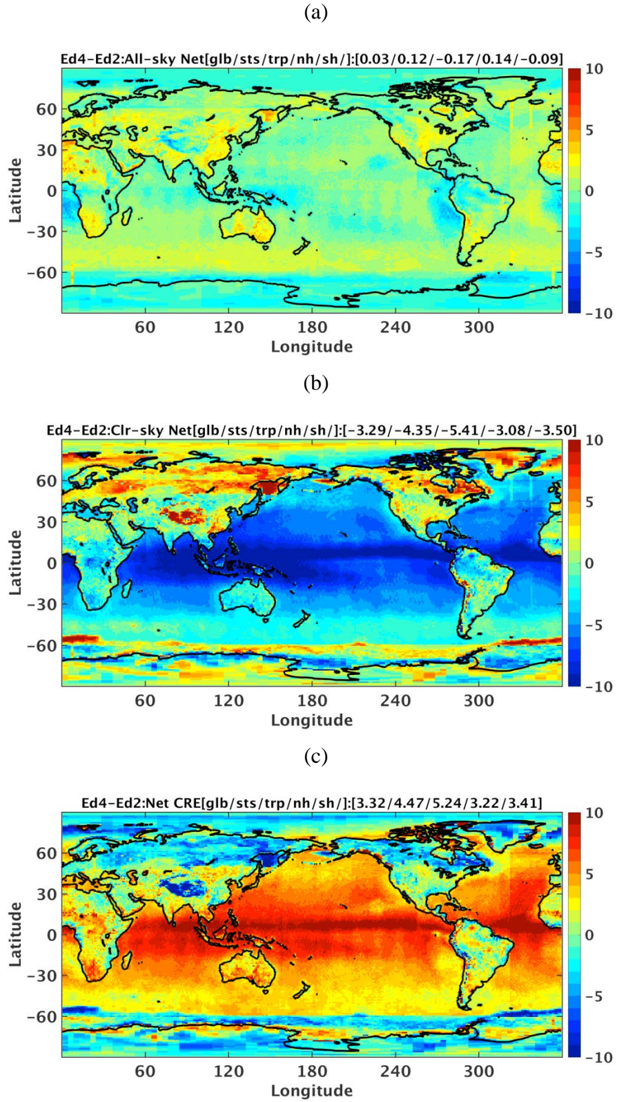
Figure 6-3. Same as Figure 6-1 but for Net.
