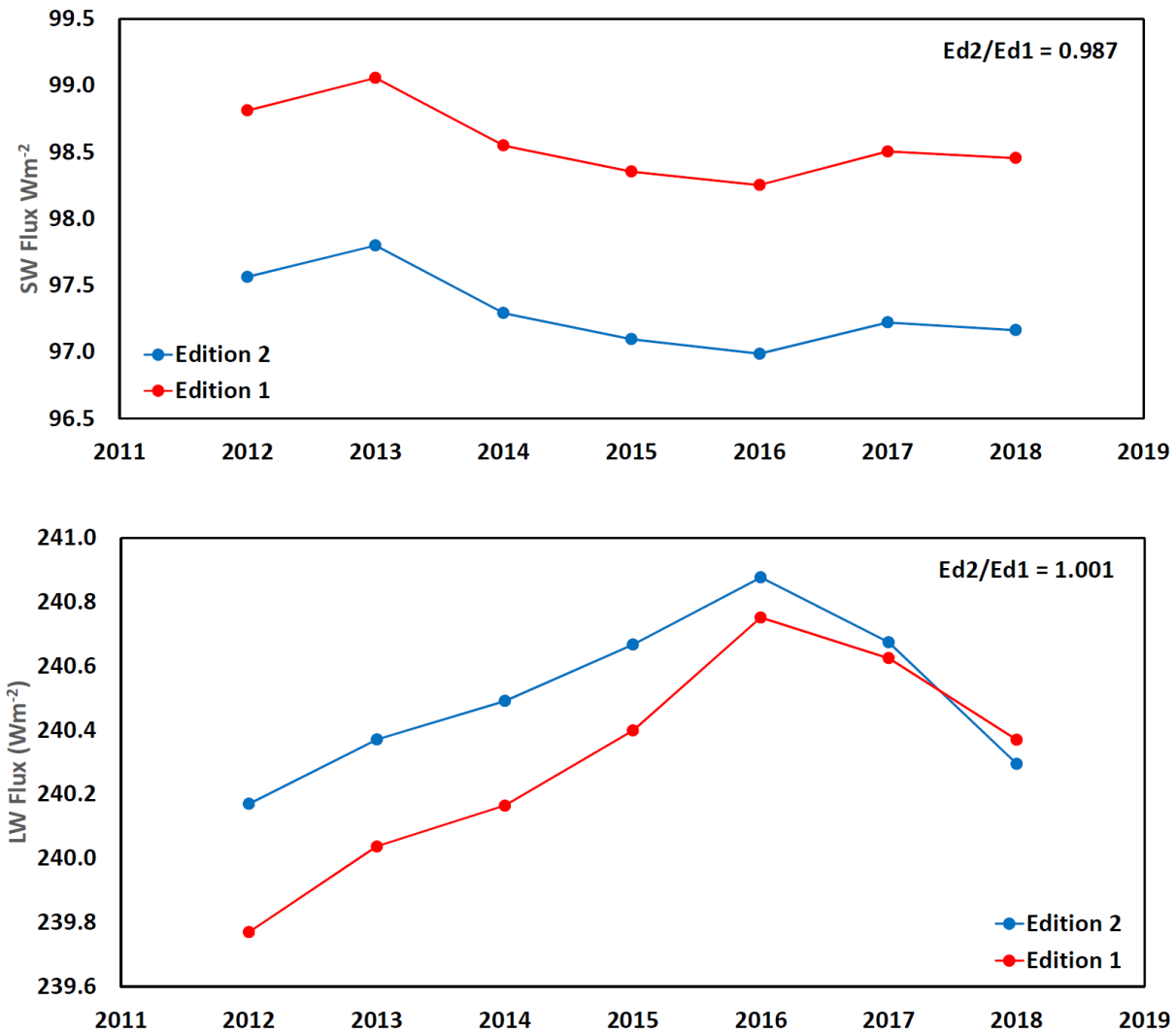
Figure 1. Time series comparisons of global annual mean NPP ES4 all-sky fluxes
