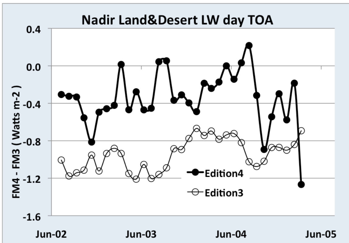
Figure 2-1. Time series of nadir-only daytime Land and Desert LW fluxes for Editions3 and 4.
