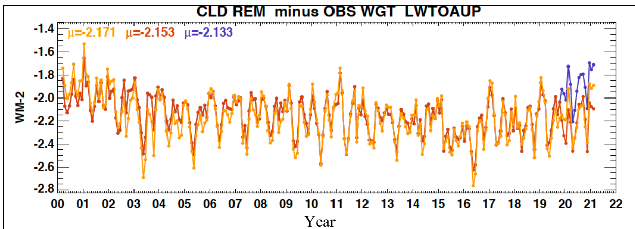
Figure 2-4. Time series of TOA upward longwave \Delta^c before the correction (blue line), after the correction (red line), and \Delta^c computed with MERRA-2 TOA upward longwave fluxes (orange line).
