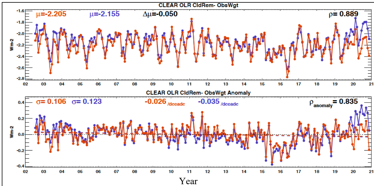
Figure 2-3. Top) Time series of the difference of global monthly mean TOA longwave flux with cloud removed and averaged by weighting by observed clear-sky fraction \Delta^c . The blue line is computed with GEOS-5.4.1 temperature and specific humidity profiles, and the red line is TOA longwave flux from MERRA-2. Bottom) monthly deseasonalized anomaly time series of the top plot. Deviation of anomalies with GEOS-4.5.1 from those from MERRA-2 from November 2019 onward is evident.
