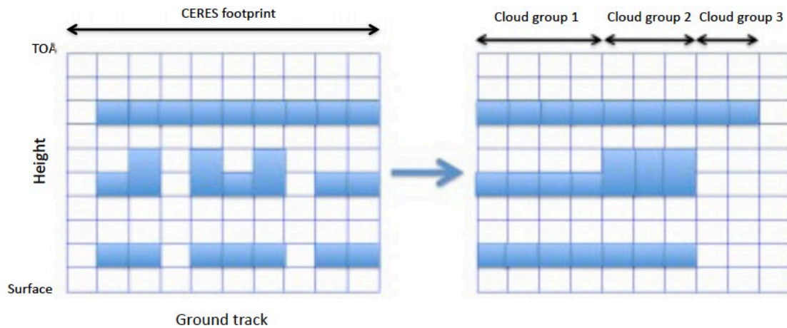
Figure 1-1. Schematic of the cloud grouping process. Cloud profiles that occur within a CERES footprint and have the same cloud boundary heights are grouped together. Group number of 1 is assigned to the cloud group having the largest cloud fraction over a CERES footprint.
