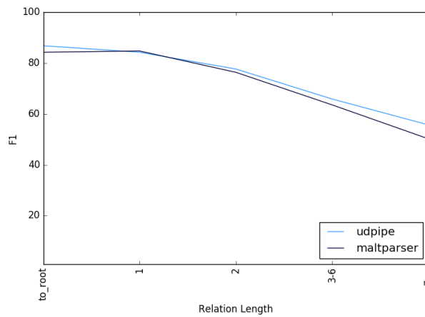
Figure 3: Accuracy relative to dependency Length
