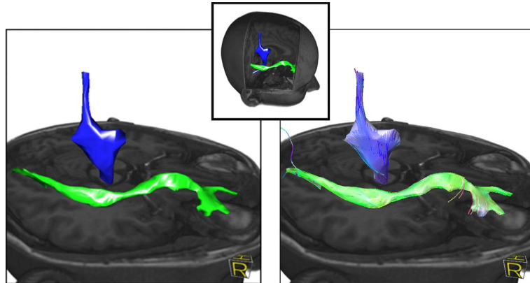
Fig. 3. Hulls obtained from tetrahedralization and 3D alpha shapes (alpha = 5): (blue) pyramidal tract, (green) optic tract, (right) combination with the fibers
