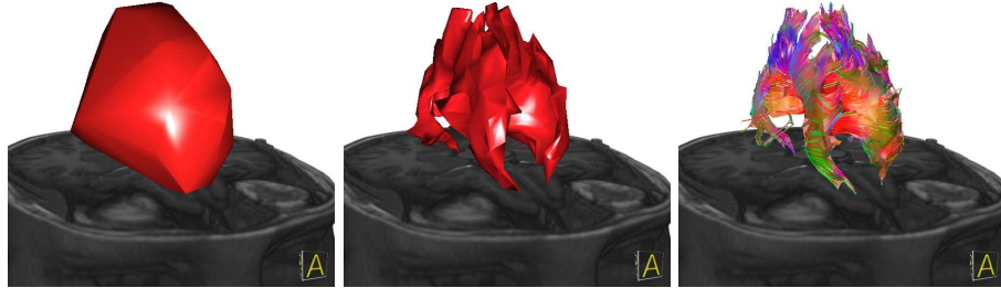
Fig. 2. 3D Delaunay tetrahedralization of a corpus callosum: (left) convex hull, (middle) subset with \alpha = 10 , (right) semi-transparent hull for \alpha = 5 displayed with tracked fibers
