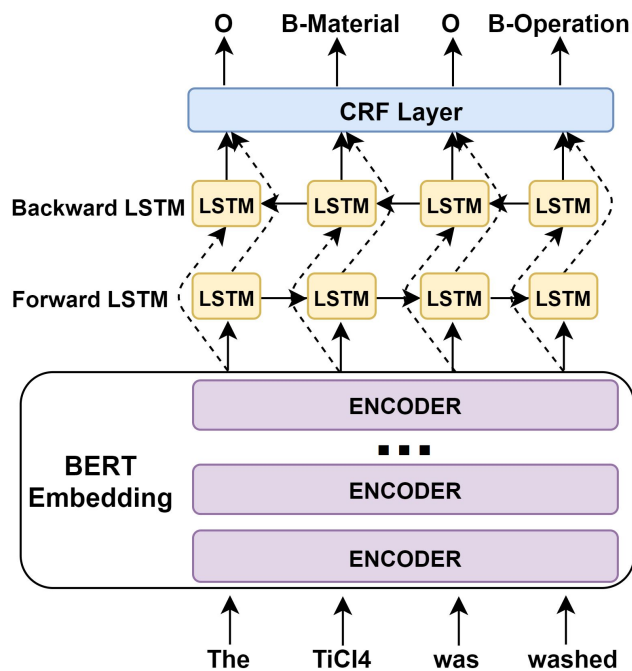
Figure 2: The architecture of the BERT-BiLSTM-CRF model.
