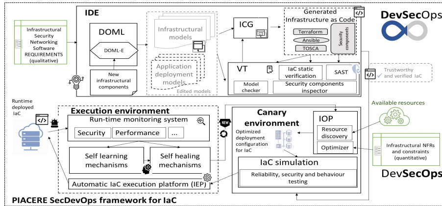
Figure 2: The PIACERE workflow.
