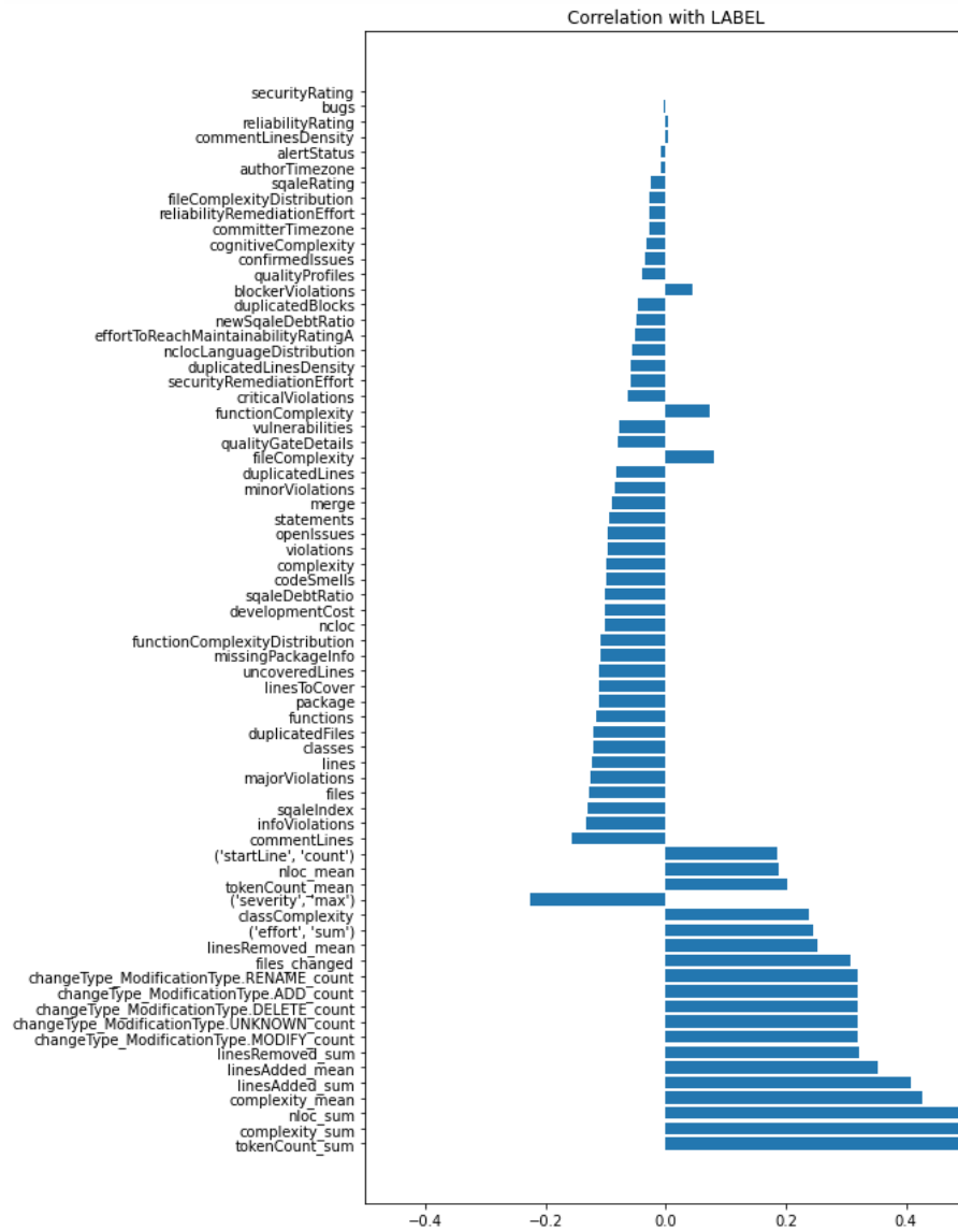
Fig. 1. List of the features with their correlation with dataset label.
