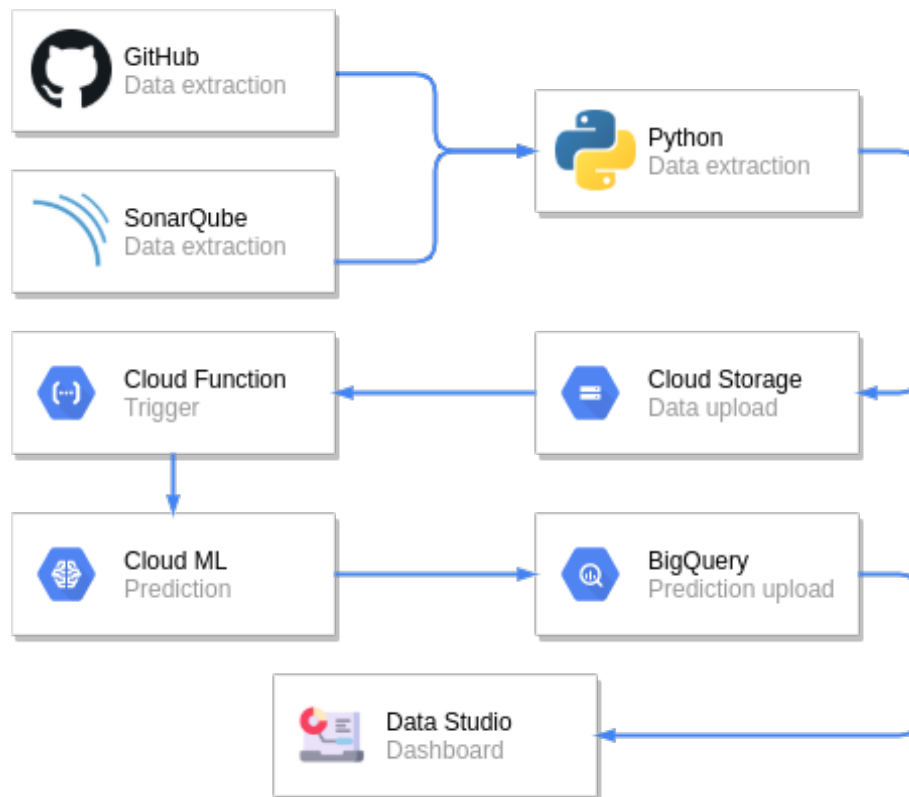
Fig. 2. Architecture of the proposed framework.
