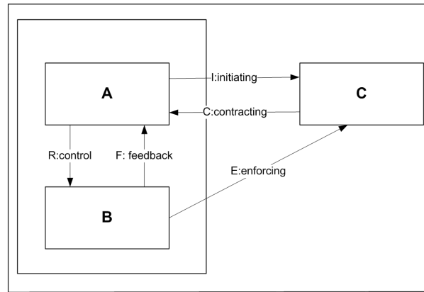
Fig. 2. Modelling Actions.
