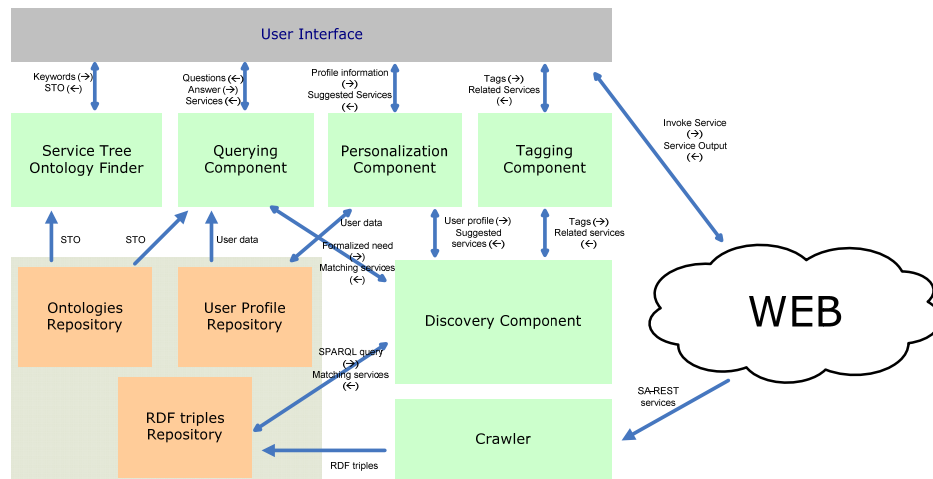
Fig. 1. Conceptual Architecture
