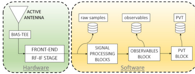
Figure 1: Software-Defined Receiver (SDR) architecture.
