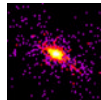
Chandra Image of NGC 4151
