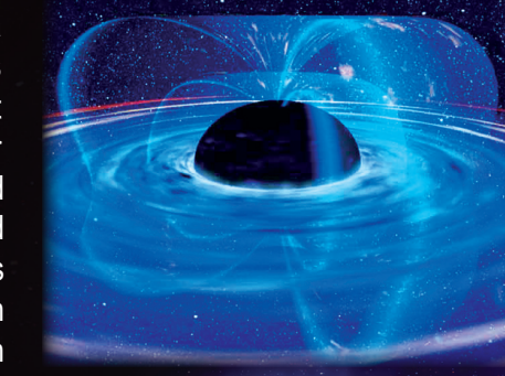
The strong magnetic field generated by the material in an accretion disk channels material onto the poles of the black hole - NASA/Dana Berry.
