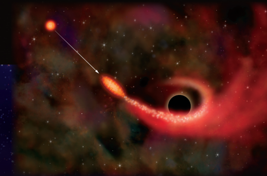
The neutron star companion of a black hole spirals in and is destroyed as it merges with the black hole - NASA/CXC/M. Weiss
