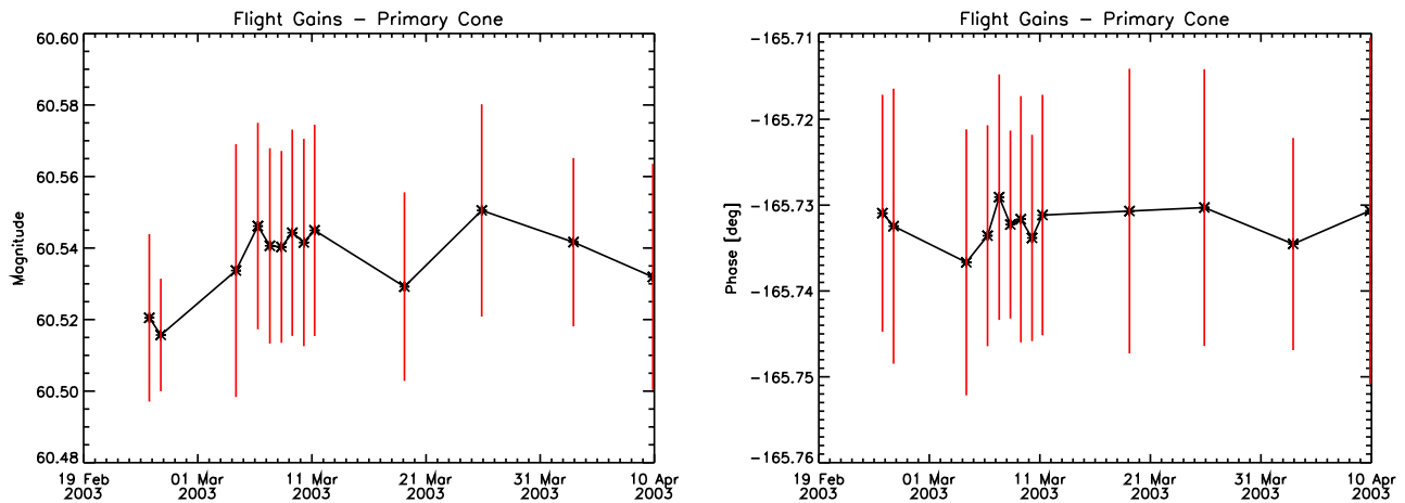
Figure 7: Gain of the primary cavity is measured at least every two weeks by analyzing the response to a DSP-provided step function. The gain magnitude (left) has relative uncertainty 4.5 \times 10^{-4} . Phase (right) is also very constant with time, again having error bars exceeding the variations.
