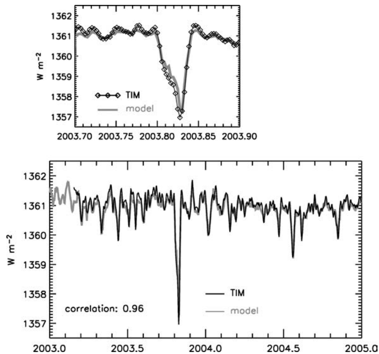
Figure 5. Shown are the TIM daily mean observations (symbols with dark line), compared with an empirical variability model developed from sunspot and facular influences (Lean, 2000). In the upper panel the observations and model are compared during the period of high solar activity in October 2003. In the lower panel the observations and model are shown for the duration of the SORCE mission thus far.
