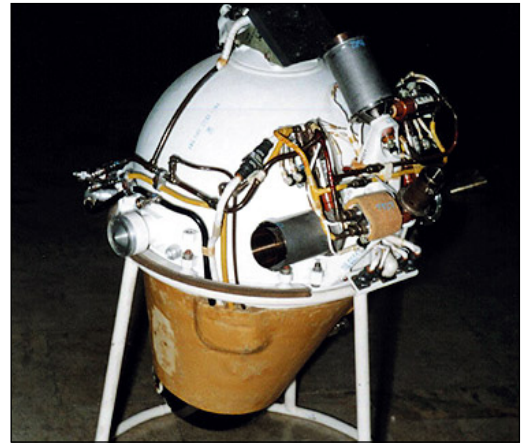
Figure 1. An 11D79 SOZ unit; nozzle assembly not installed. Photo credit: RKK Energia/Kosmonavtika.com.
