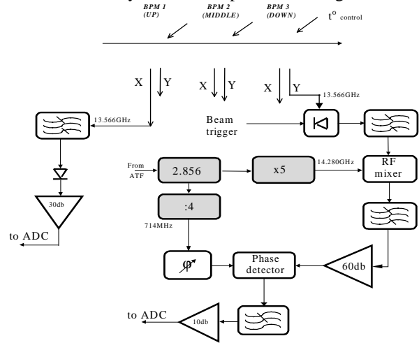
Figure 5. RF circuit.
