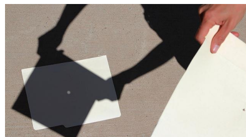
Pinhole Projection
