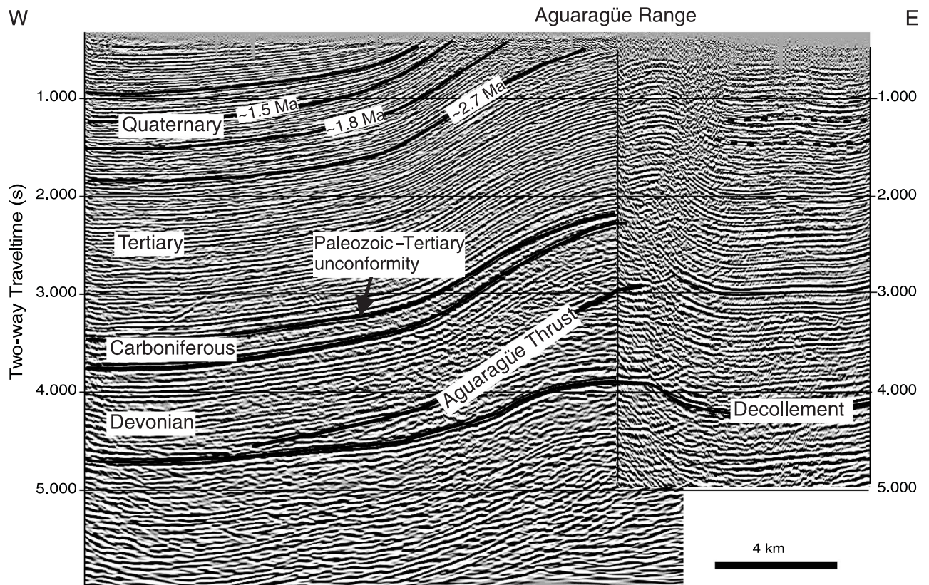
Figure 11. Uninterpreted and interpreted migrated seismic line of the Aguaragüe range. Progressive limb rotations at the back limb have been interpreted with ages of about 1–1.5 Ma. Located in Figure 2 as line 7.
