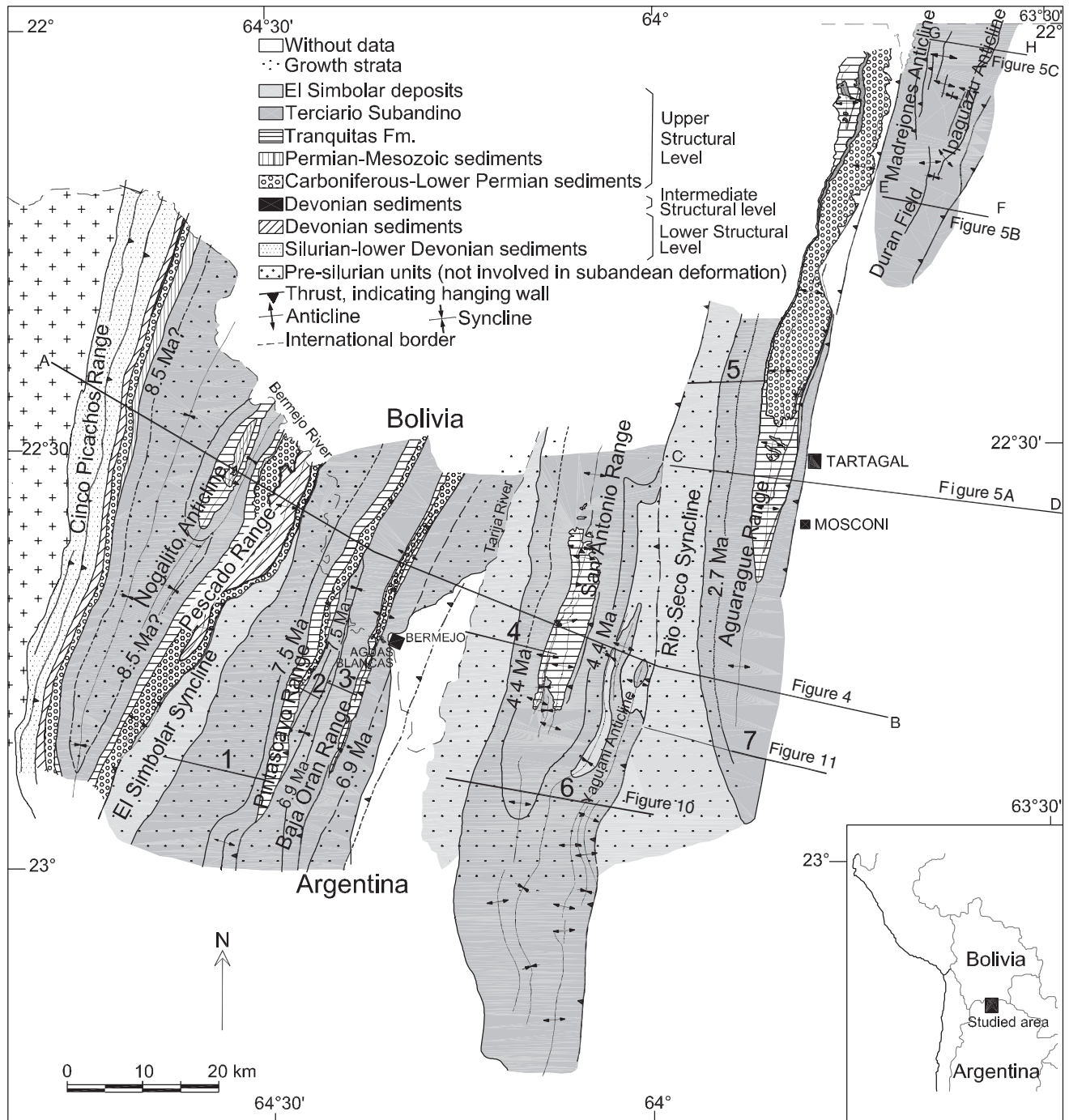
Figure 2. Location and simplified geologic map of the northwestern Argentina Subandean belt. Cross-section locations: AB, regional cross section (Figure 4); CD, Aguaragüe range cross section (Figure 5A); EF, Duran field cross section (Figure 5B); GH, Madrejonas-Ipaguazu field cross section (Figure 5C). Magnetic-polarity stratigraphy section (Figure 7) locations: (1) Río Iruya; (2) Las Manzanas; (3) Peña Colorada; (4) La Porcelana; (5) Quebrada de León. Seismic lines location: (6) San Antonio range seismic line (Figure 10); (7) Aguaragüe range seismic line (Figure 11).
