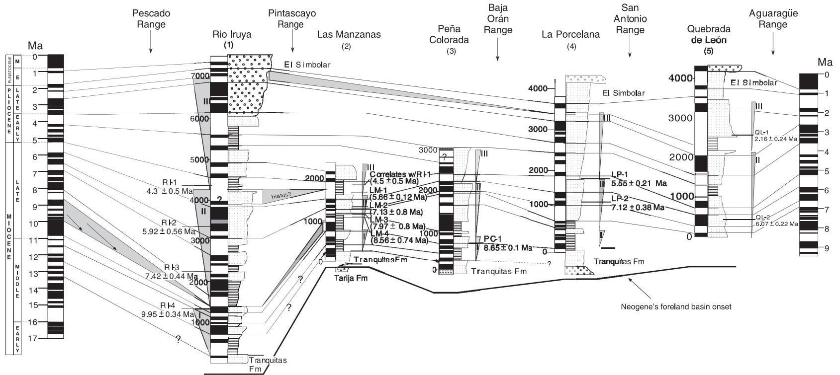
Figure 7. Correlation of the Río Iruya, Peña Colorada, Las Manzanas, La Porcelana, and Quebrada de León magnetic-polarity stratigraphy with the magnetic polarity timescale of Cande and Kent (1995). Positions in each column of isotopically dated volcanic ash are also shown. See Figure 2 for location of the five stratigraphic sections. Vertical scales posted on stratigraphic columns are in meters.
