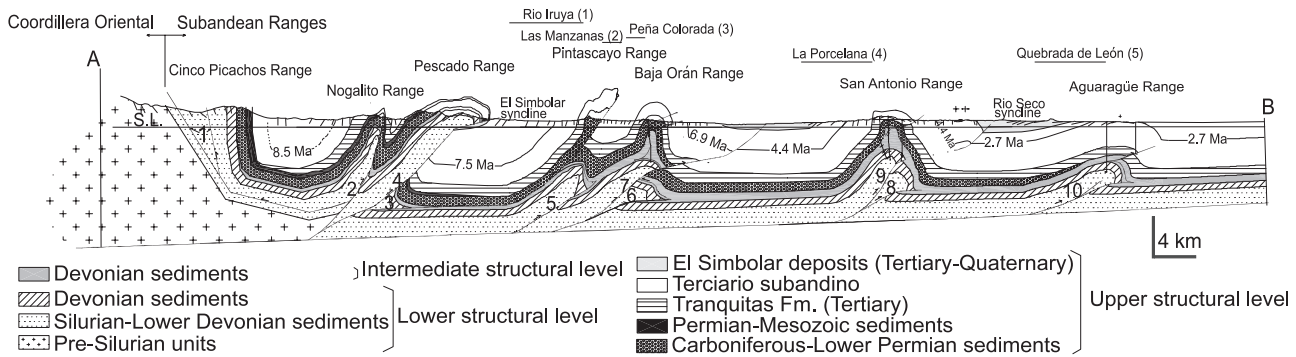
Figure 4. Balanced cross section across the entire Subandean thrust and fold belt. (1) Cinco Picachos back thrust; (2) Nogalito thrust: in-sequence with out-of-sequence reactivation; (3) Pescado thrust: in-sequence; (4) Pescado thrust: out-of-sequence; (5) Pintascayo thrust: in-sequence with out-of-sequence reactivation; (6) Baja Orán thrust: in-sequence; (7) Baja Orán thrust: out-of-sequence; (8) San Antonio thrust: in-sequence; (9) San Antonio thrust: out-of-sequence; (10) Aguaraquí thrust: in-sequence (with minor out-of-sequence reactivation?). The time lines shown in the Tertiary (based on volcanic ash geochronology and magnetic-polarity stratigraphy) represent the local boundary between the pregrowth and growth strata. Positions of magnetic-polarity stratigraphy sections are also shown. See Figure 2 for location. No vertical exaggeration.
