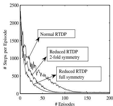
Figure 3: Learning curves for the Deterministic Grid World(25x25 grid).
