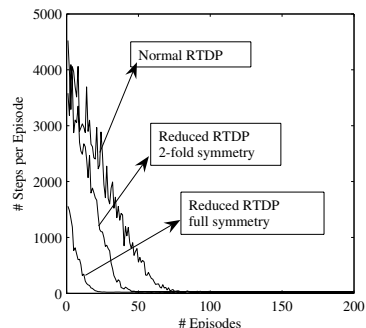
Figure 5: Learning curves for the Probabilistic Towers of Hanoi(5 disks).
