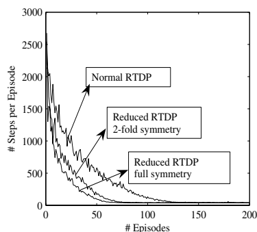
Figure 4: Learning curves for the Probabilistic Grid World(25x25 grid).
