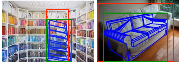
Figure 8. Corner cases: these two images illustrate cases which are incorrect under our pose estimation criteria, but are still correct under standard bounding box detection criterion.
