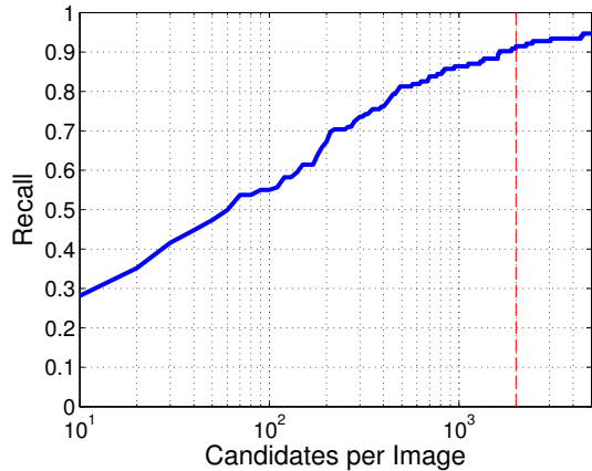
Figure 7. RANSAC evaluation: we evaluated how many pose candidates per image we need in order to obtain a certain recall. We need only about 2000 candidates in order to have 0.9 recall. This allows us to perform a computationally expensive feature extraction on only a small number of candidates.
