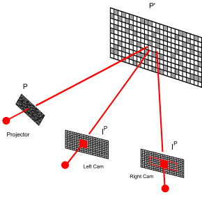
Fig. 2. Our projector and stereo camera system. A pattern P is projected onto a surface to produce P' , which is imaged by a left and right camera. To compute depth, the small red block in the left image is matched against a range of blocks in the right image at the same vertical offset, indicated by the outlined rectangle.
