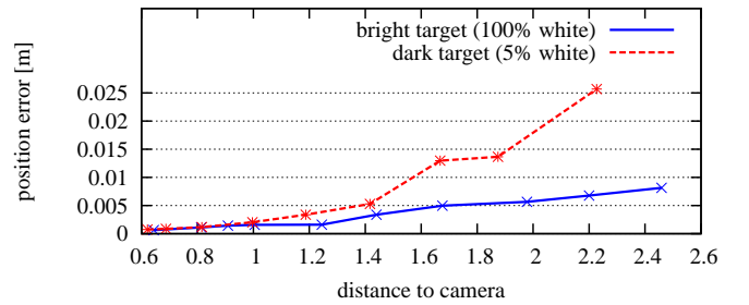
Fig. 3. Positional error of a planar target, observed with our active stereo camera system. For a white target, the error stays below 2mm until after 1.2m, then goes up to about 1cm at 2.5m. For a very dark target, error is low close up, then becomes larger at distance, when the pattern is difficult to see.
