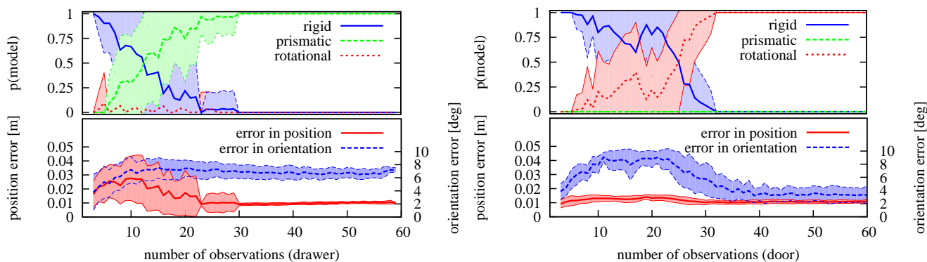
Fig. 12. Evaluation of the articulation models learned for the drawer (left) and the door (right), averaged over 50 runs. The plots at the top show the probability of the articulation model templates, the plots at the bottom show the prediction error of the learned model.
