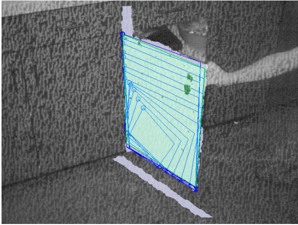
Fig. 6. In each plane, we pick a random starting point from which we optimize iterative the pose and size of the candidate rectangle. In this case, the found rectangle is accepted because both r_{\text{recall}} and r_{\text{precision}} are high enough (see text).
