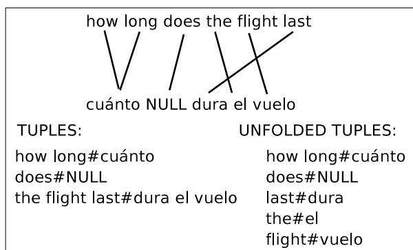
Figure 1: Comparing regular and unfolded tuples.
