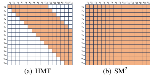
(a) HMT (b) SM 2 (c) Effect of prohibition to the SiMT performance.
