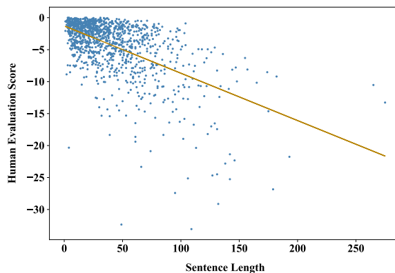
Figure 3: The correlation between sentence lengths (x-axis) and human average translation scores (y-axis) on WMT23 Chinese-English dataset for the metric shared task.
