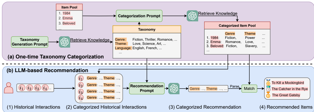
Figure 2: The proposed TAXREC for zero-shot LLM-based recommendation. (a) One-time Taxonomy Categorization step aims to generate in-domain taxonomy and enrich/categorize item’s title into structured text information. (b) LLM-based Recommendation step provides ranked item lists for users based on the user’s historical interactions.
