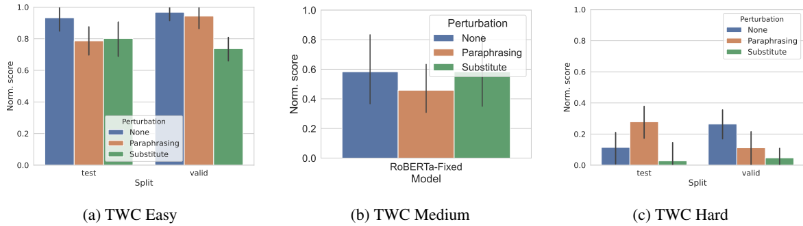
Figure 9: Evaluation of an RoBERTa agent on original, paraphrased, and lexical substitution observations on (a) Easy, (b) Medium and (c) Hard games.
