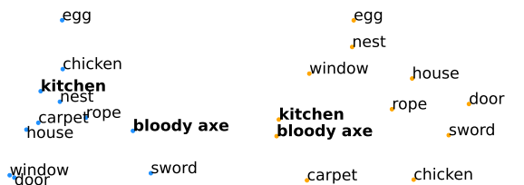
Figure 5: Shift caused by the semantic degeneration to the contextual word vectors in the RoBERTa model fine-tuned to Zork 1 : (a) pre-trained embeddings, (b) embeddings fine-tuned to Zork 1 . Bolded words denote the case where the term “bloody axe” shifts towards the word “kitchen” as a result of them co-occurring in a positively rewarded state.
