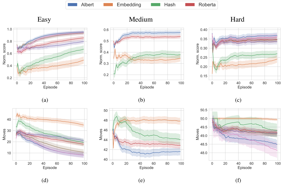
Figure 8: Comparison of the performance across several language encoding models. Figures a, b, c show the normalized score for easy, medium and hard games, respectively. Figures d, e, f show the number of movements needed by the agent to complete the task (lower values are better). Shaded region corresponds one standard deviation.
