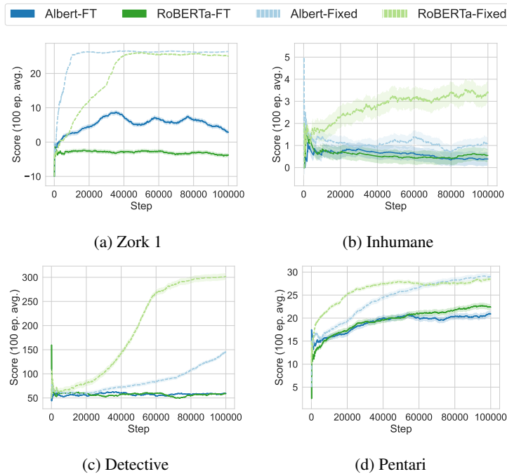
Figure 4: Training comparison of fine-tuned/fixed LMs on four Jericho games.
