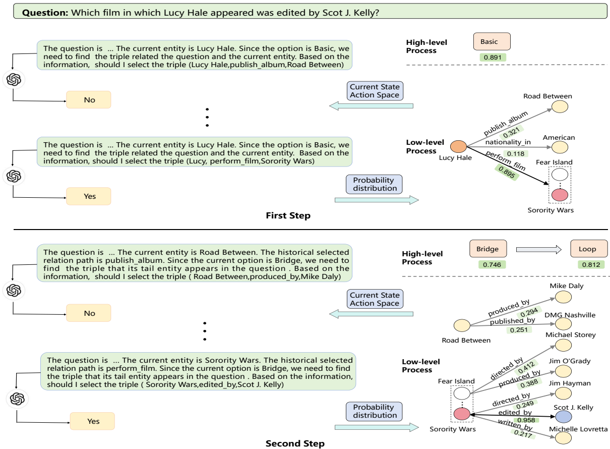
Figure 3: A case of the hierarchical decision process.
