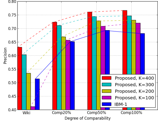
Figure 4: Robustness of method under different data conditions.
