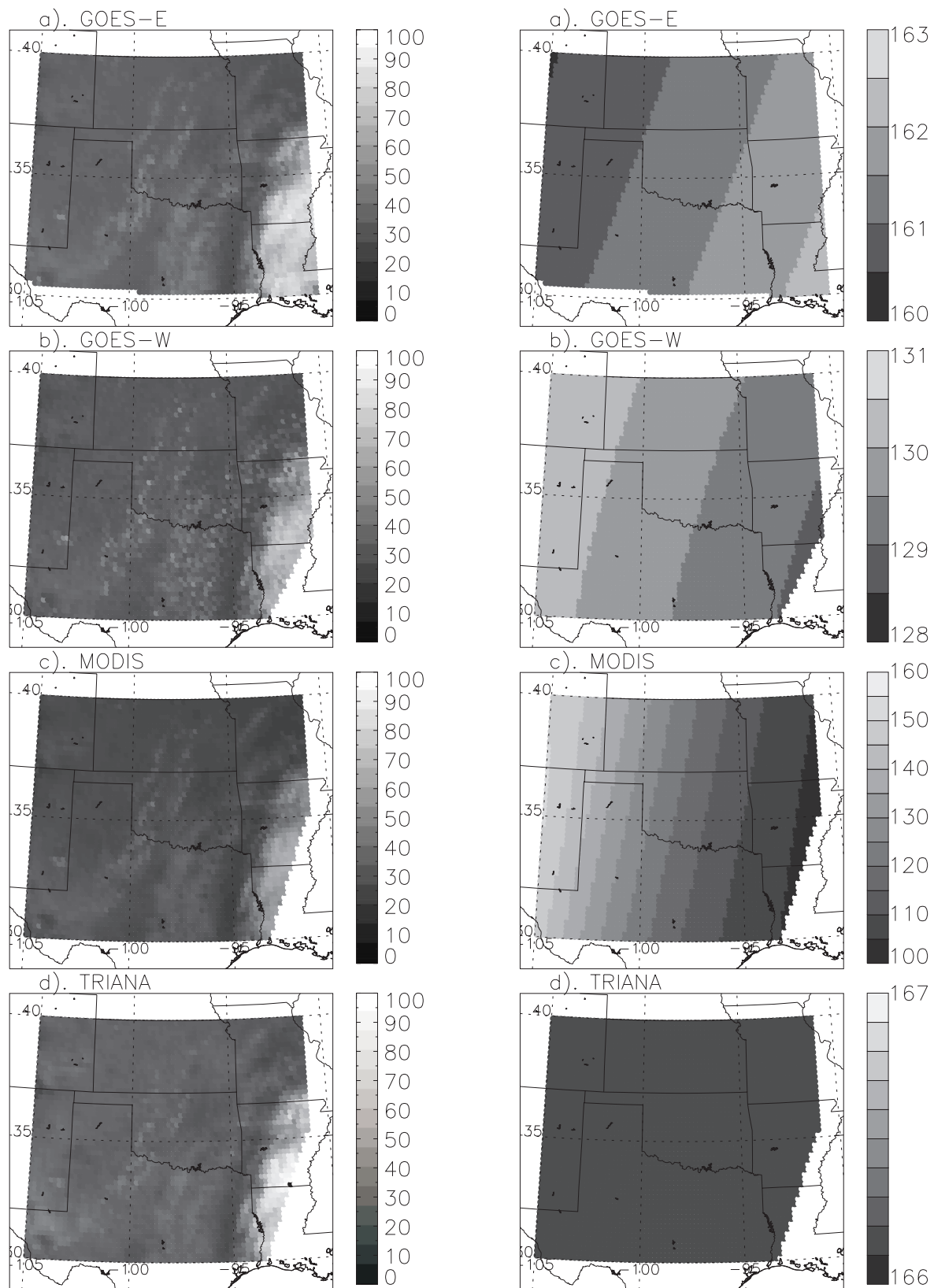
Figure 2. Matched satellite VIS imagery (left) and scattering angles (right, in degree), 1800 UTC, September 7, 2000.
