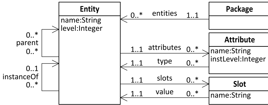
Figure 3: Minimal Metamodel for Multi-level Modelling
