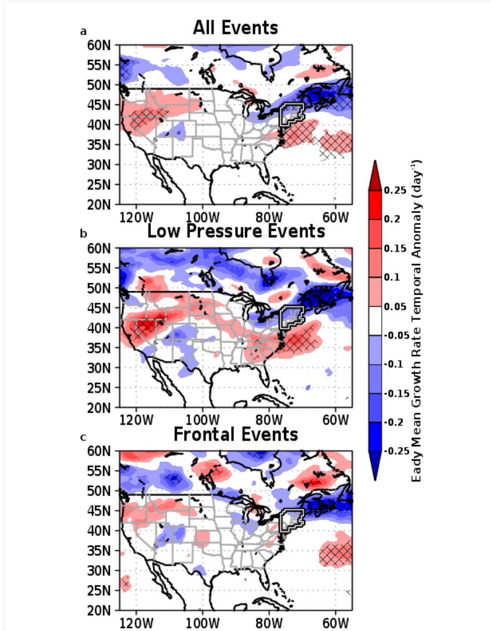
Figure 4. The difference in Eady mean growth rate on the day of an extreme precipitation event in the Northeastern United States during 1997 through 2014 and 1980 through 1996 for (a) all events, (b) events caused by a low pressure system, and (c) events caused by frontal systems. Hatching denotes areas with a statistical significance of 95 percent.
