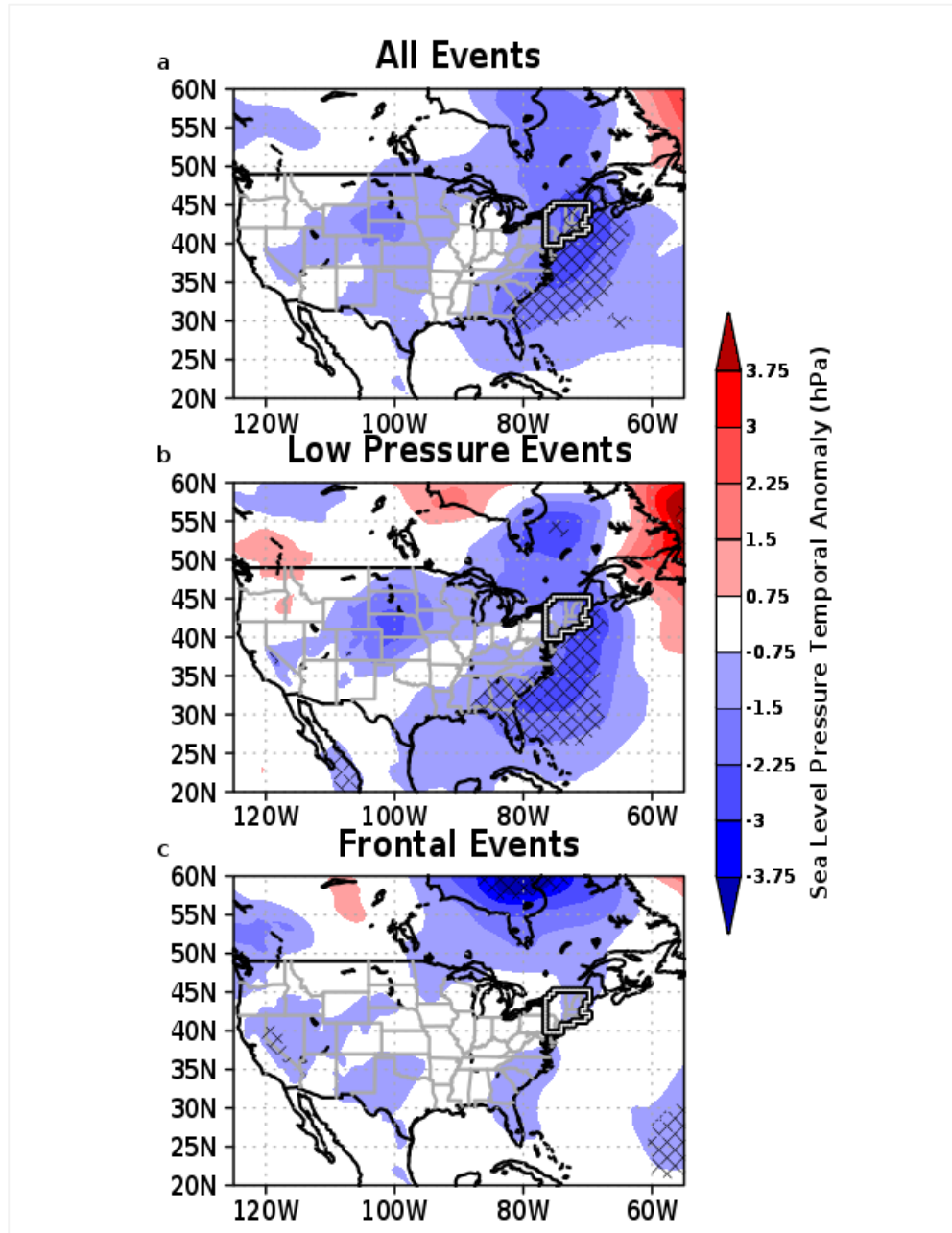
Figure 2. The difference in sea level pressure during observed extreme precipitation events in the Northeastern United States during 1997 through 2014 and 1980 through 1996 for (a) all events, (b) events caused by a low pressure system, and (c) events caused by frontal systems. Hatching denotes areas with a statistical significance of 95 percent.
