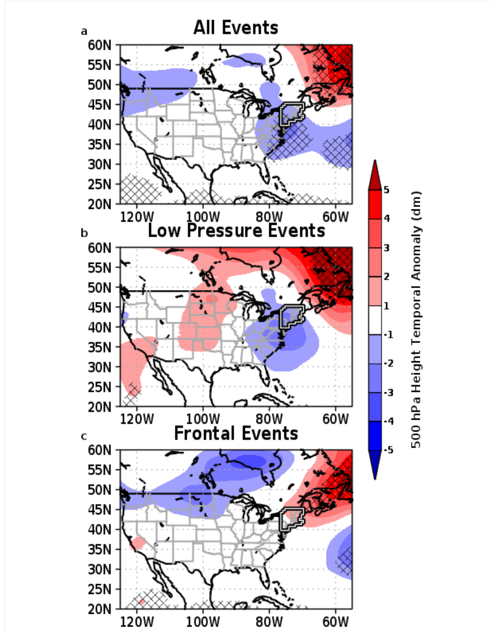
Figure 3. The difference in 500 hPa height on the day of an extreme precipitation event in the Northeastern United States during 1997 through 2014 and 1980 through 1996 for (a) all events, (b) events caused by a low pressure system, and (c) events caused by frontal systems. Hatching denotes areas with a statistical significance of 95 percent.
