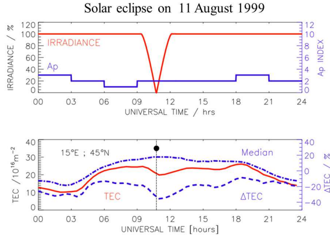
Fig. 5.16. Ionospheric depletion of the total ionization of the ionosphere (TEC) in the zone of totality at 15^{\circ}\text{E} ; 45^{\circ}\text{N} during the solar eclipse on 11 August 1999 in comparison with the corresponding monthly median TEC.
