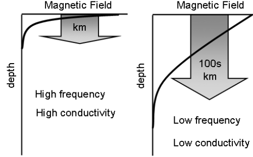
Fig. 4.5. Penetration of magnetic fields into the Earth
