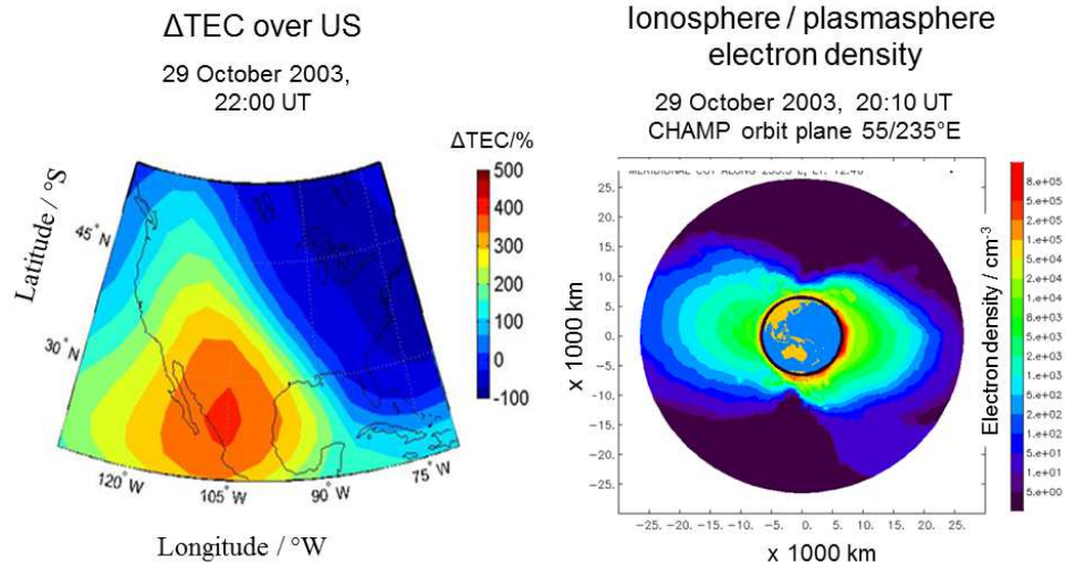
Fig. 5.19. Percentage deviations of TEC over US from corresponding monthly medians on 29 October 2003 at 22:00 UT (left panel). Topside reconstruction of the electron density distribution in the CHAMP orbit plane for 29 October 2003 around 20:10 UT (right panel).
