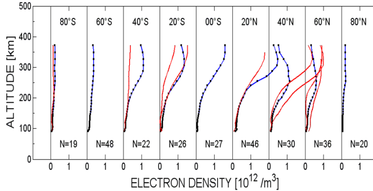
Fig. 5.20. IRO retrieved electron density profiles for 15°E longitude and different latitude zones on October 29, 2003 (red line). Comparison is made with corresponding median profiles, number N of profiles used for calculation is given.
