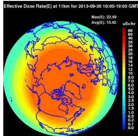
Fig. 3.1. NAIRAS effective dose rate at the time of the U.S. Government shutdown of NASA LaRC computers and prior to the 20:05 UT peak of the radiation storm on September 30, 2013. Courtesy of Space Environment Technologies and NASA Langley Research Center NAIRAS project.
