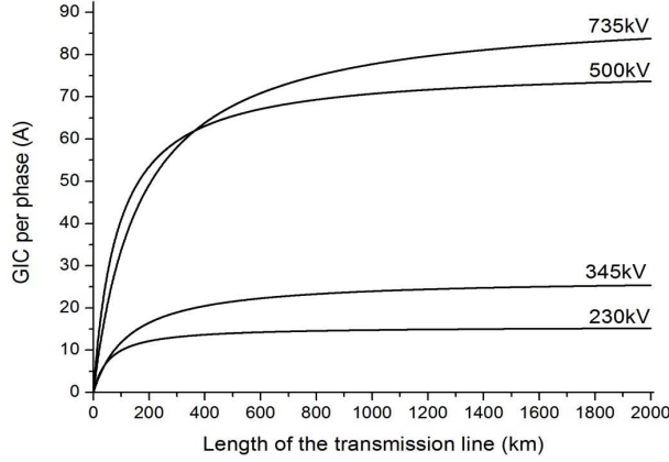
Fig. 4.11. GIC dependence on line length (from Zheng et al., 2013).
