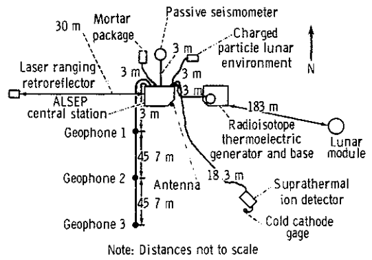
Figure 1-3.- Deployment configuration for Apollo 14 ALSEP.
