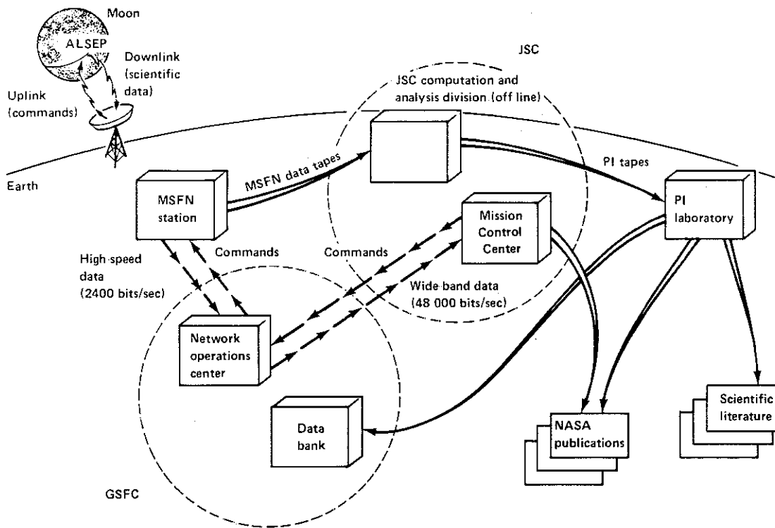
Figure 3-1.- ALSEP communication network.
