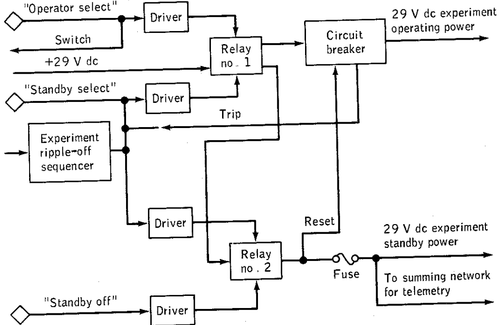
Figure 2-12.- Power control circuit for typical ALSEP experiment.
