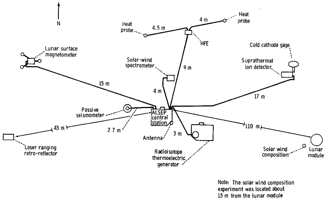
Figure 1-4.- Deployment configuration for Apollo 15 ALSEP.
