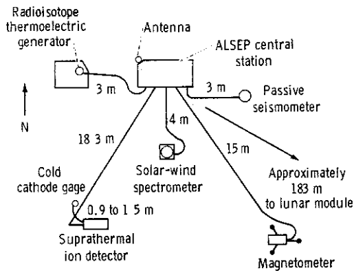
Figure 1-2.- Deployment configuration for Apollo 12 ALSEP.
