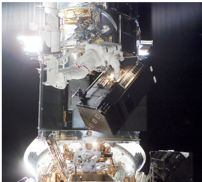
Astronauts James H. Newman (on the remote manipulator system robotic arm) and Michael J. Massimino install ACS during Servicing Mission 3B.
