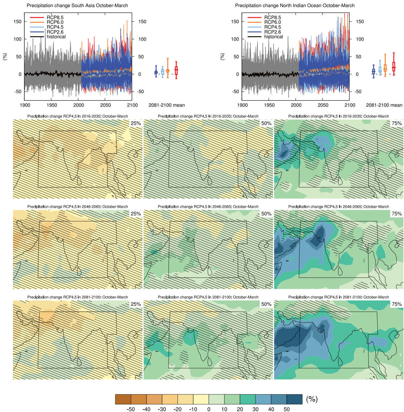
Figure AI.62 | (Top left) Time series of relative change relative to 1986–2005 in precipitation averaged over land grid points in South Asia (60°E, 5°N; 60°E, 30°N; 100°E, 20°E; 95°E, 20°N; 95°E, 5°N) in October to March. (Top right) Same for sea grid points in the North Indian Ocean (5°N to 30°N, 60°E to 95°E). Thin lines denote one ensemble member per model, thick lines the CMIP5 multi-model mean. On the right-hand side the 5th, 25th, 50th (median), 75th and 95th percentiles of the distribution of 20-year mean changes are given for 2081–2100 in the four RCP scenarios.
