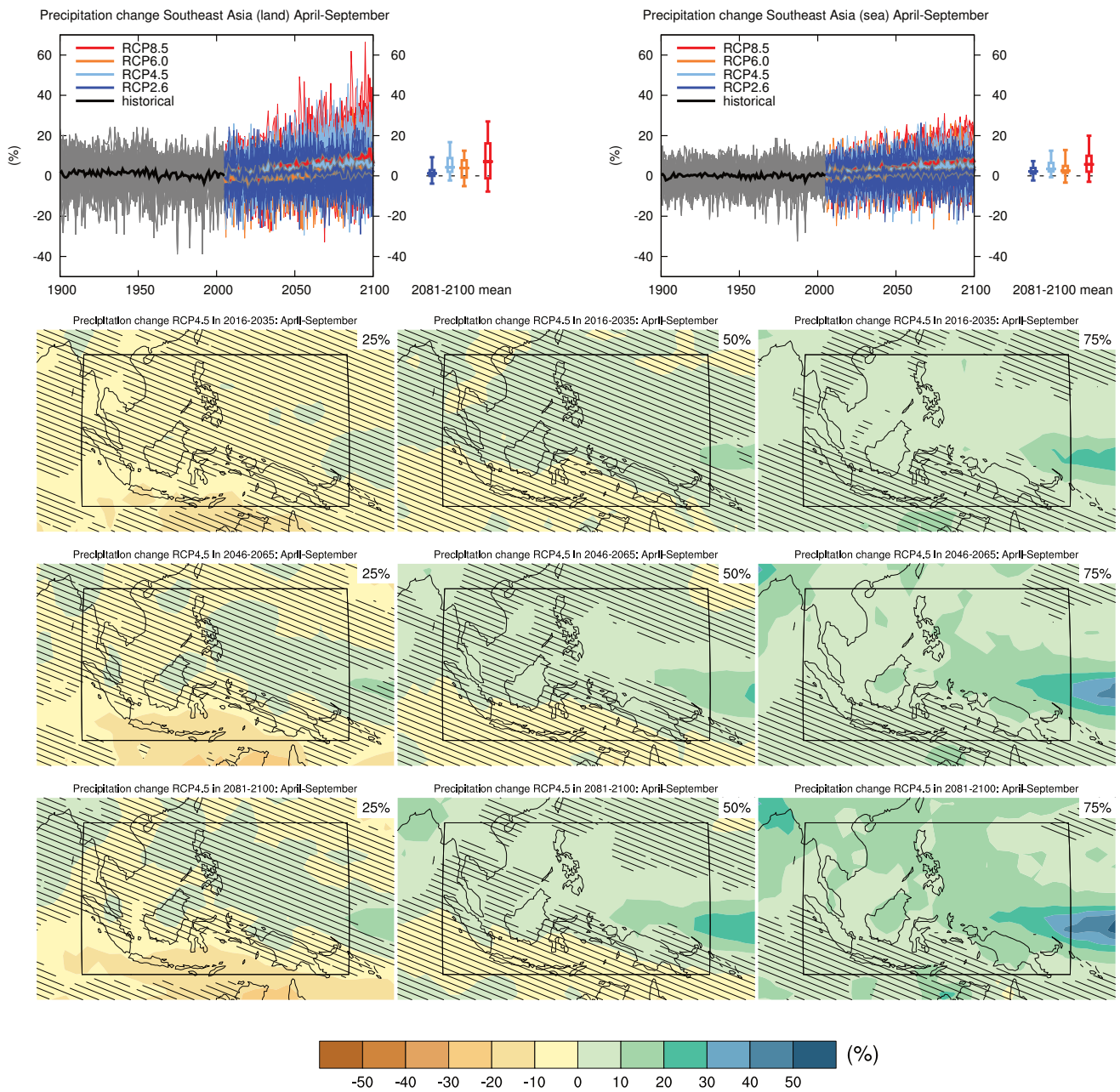
Figure AI.67 | (Top left) Time series of relative change relative to 1986–2005 in precipitation averaged over land grid points in Southeast Asia (10°S to 20°N, 95°E to 155°E) in April to September. (Top right) Same for sea grid points. Thin lines denote one ensemble member per model, thick lines the CMIP5 multi-model mean. On the right-hand side the 5th, 25th, 50th (median), 75th and 95th percentiles of the distribution of 20-year mean changes are given for 2081–2100 in the four RCP scenarios.
