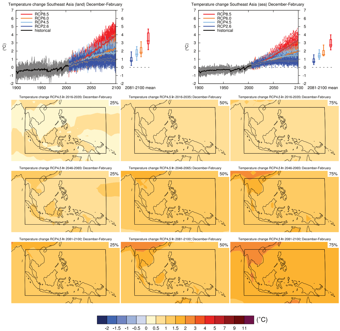
Figure AI.64 | (Top left) Time series of temperature change relative to 1986–2005 averaged over land grid points in Southeast Asia (10°S to 20°N, 95°E to 155°E) in December to February. (Top right) Same for sea grid points. Thin lines denote one ensemble member per model, thick lines the CMIP5 multi-model mean. On the right-hand side the 5th, 25th, 50th (median), 75th and 95th percentiles of the distribution of 20-year mean changes are given for 2081–2100 in the four RCP scenarios.
